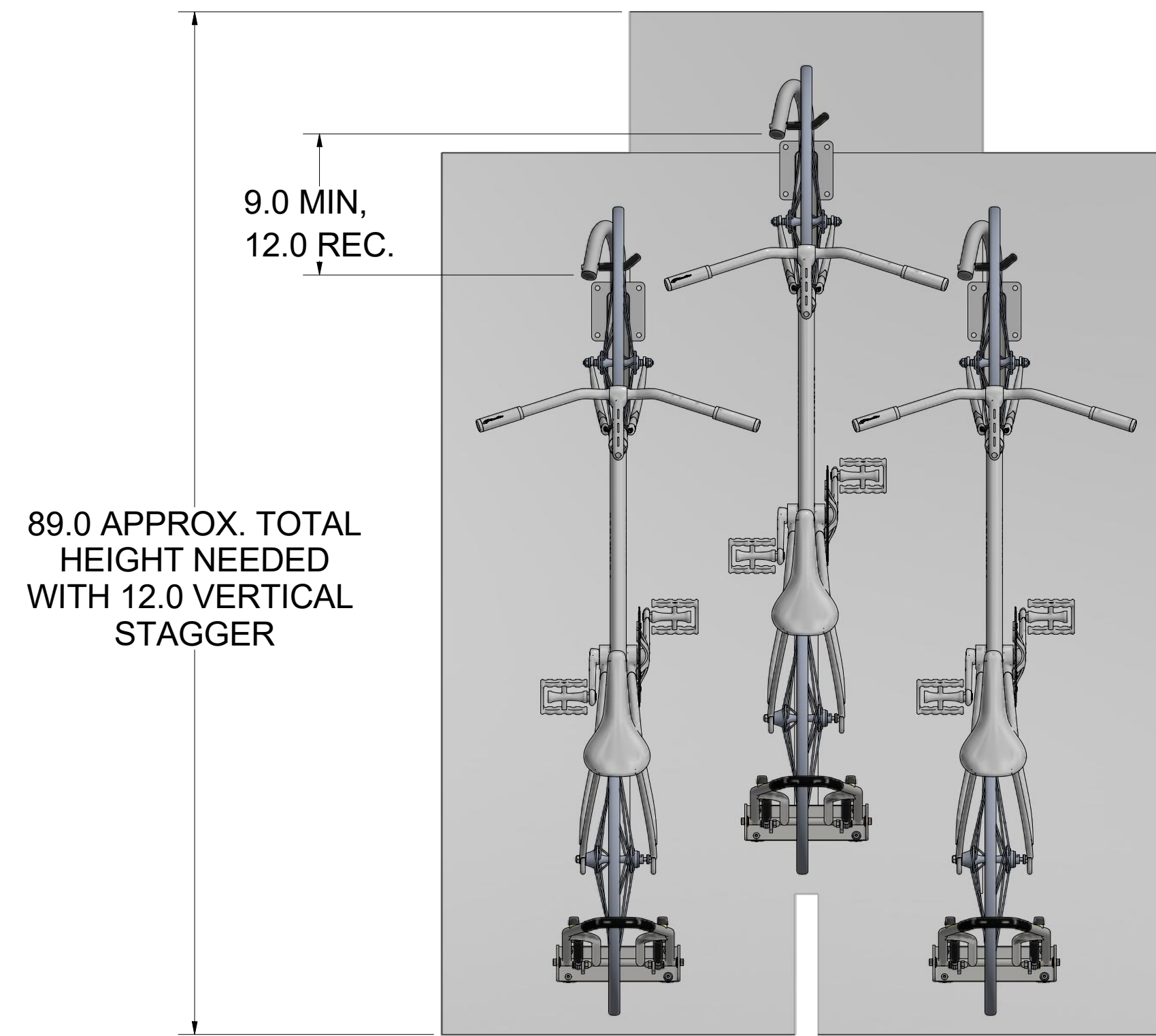
16" SPACING WITH 12" VERTICAL STAGGER
